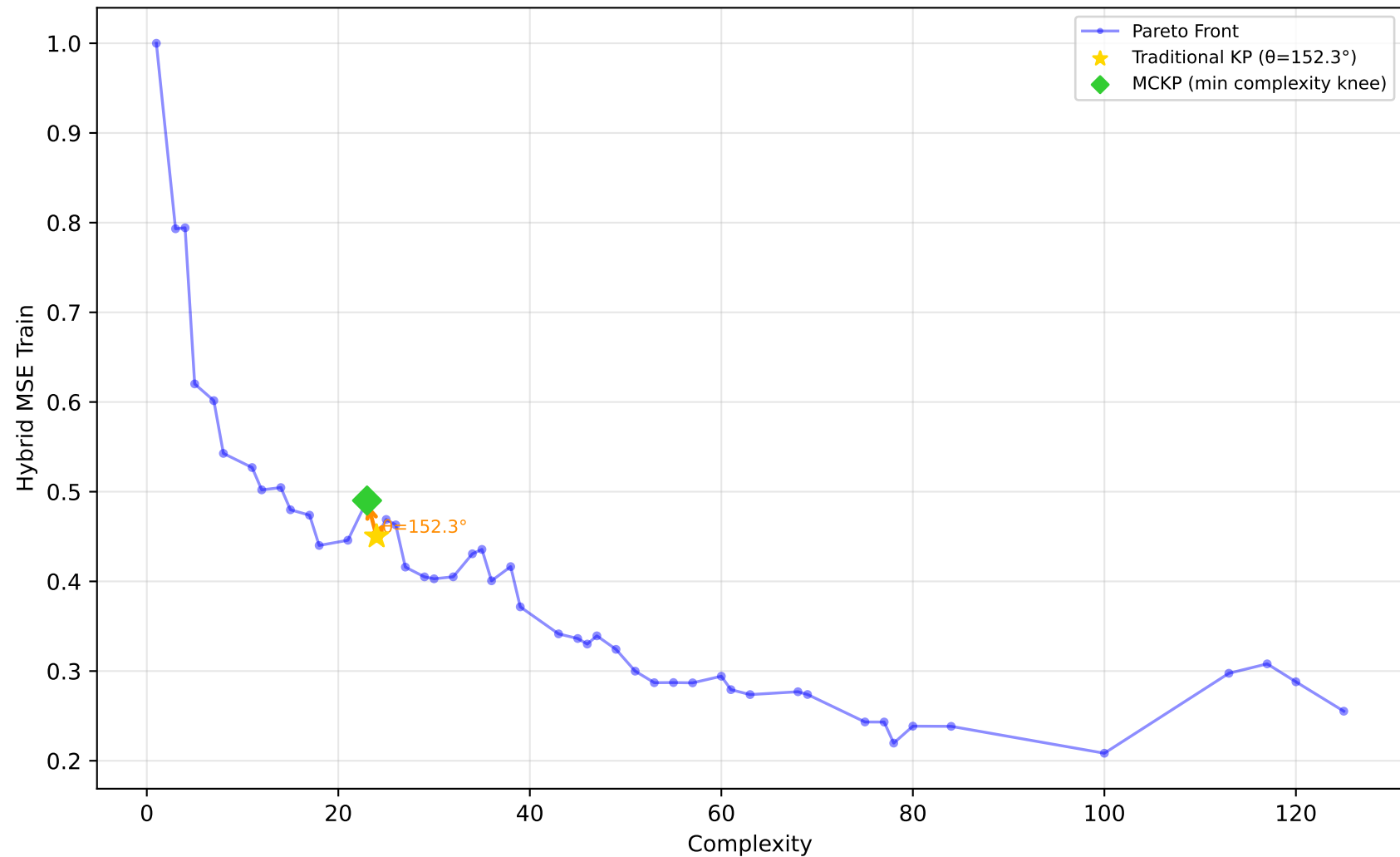
192_vineyard - Run 2 - SVP - Hybrid MSE Train \lambda_1=0.70, \lambda_2=0.70, \lambda_3=0.90 | Difficulty: 0.13 | Method: mckp
