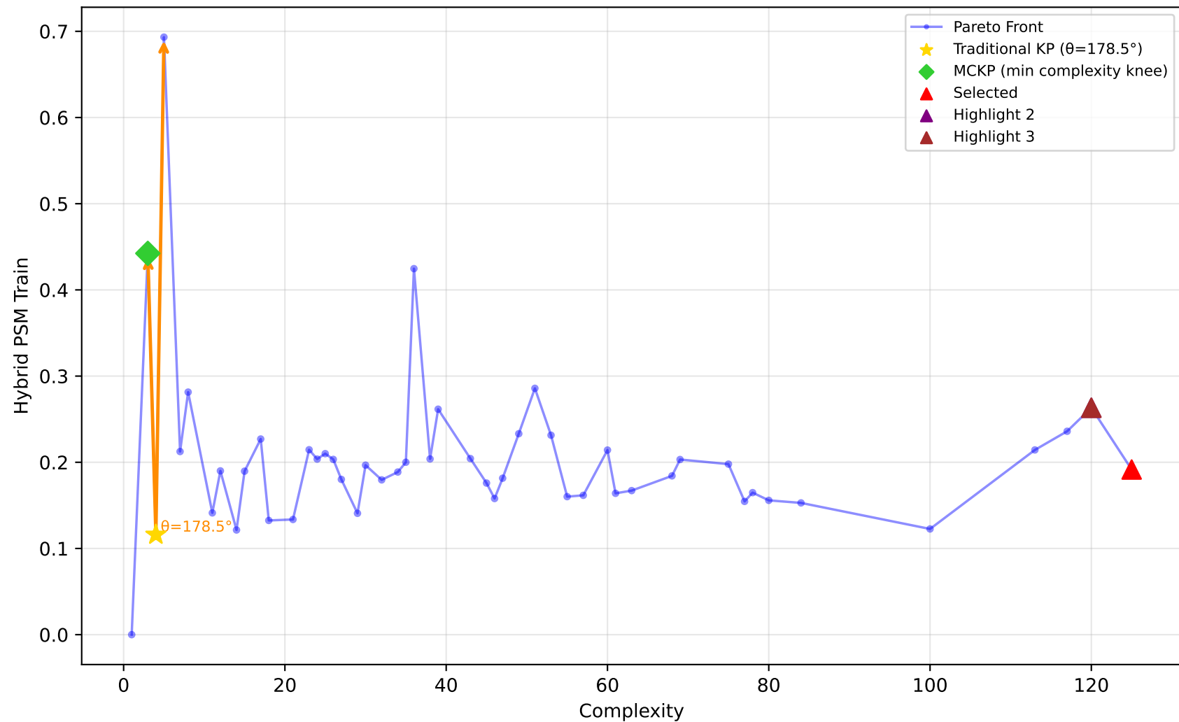
192_vineyard - Run 2 - SVP - Hybrid PSM Train \lambda_1=0.70, \lambda_2=0.70, \lambda_3=0.90 | Difficulty: 0.13 | Method: mckp
