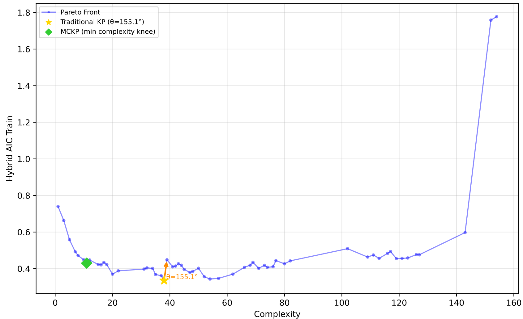
192_vineyard - Run 30 - MVP - Hybrid AIC Train \lambda_1=0.40, \lambda_2=0.00, \lambda_3=1.00 | Difficulty: 0.67 | Method: hmr
