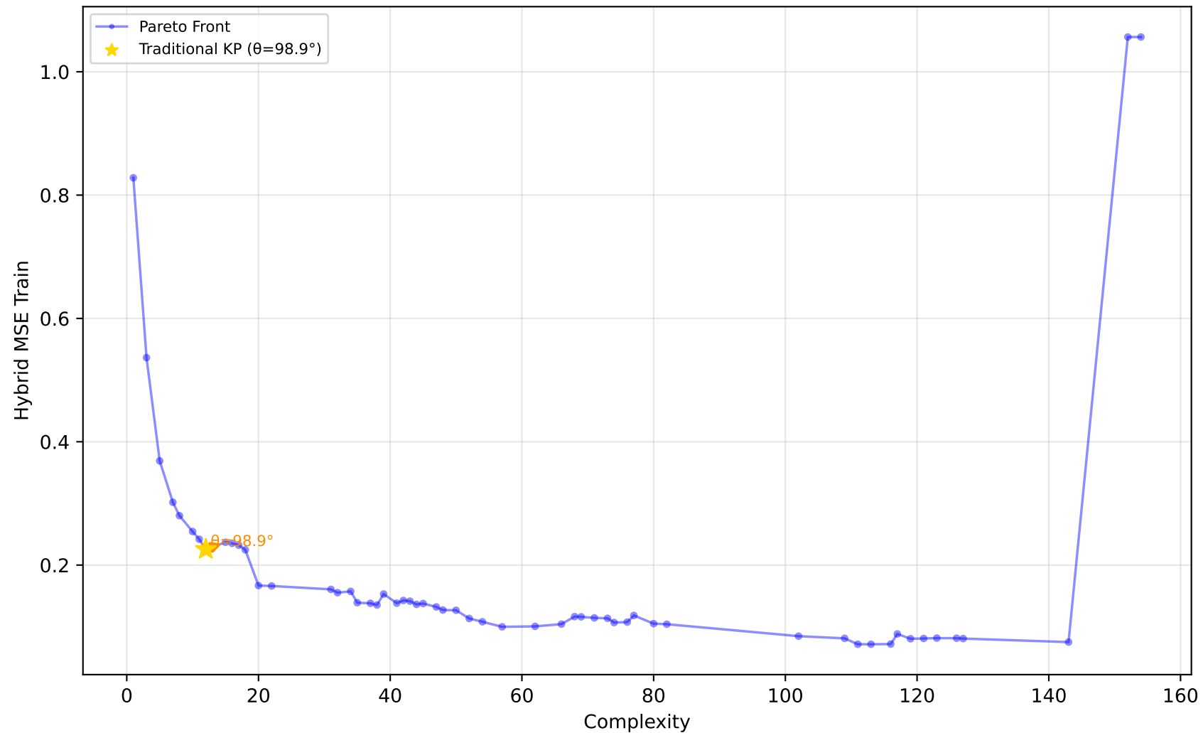
192_vineyard - Run 30 - MVP - Hybrid MSE Train \lambda_1=0.00, \bar{\lambda}_2=0.30, \lambda_3=1.00 | Difficulty: 0.67 | Method: hmr
