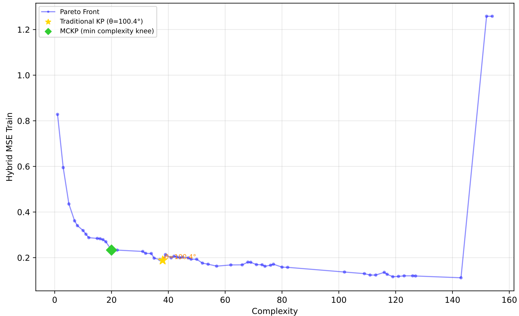
192_vineyard - Run 30 - MVP - Hybrid MSE Train \lambda_1=0.40, \bar{\lambda}_2=0.00, \lambda_3=1.00 | Difficulty: 0.67 | Method: hmr
