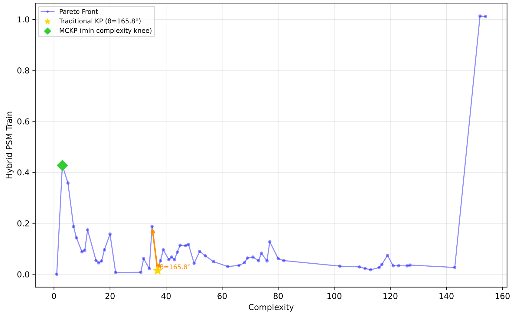
192_vineyard - Run 30 - MVP - Hybrid PSM Train \lambda_1=0.00, \bar{\lambda}_2=0.30, \lambda_3=1.00 | Difficulty: 0.67 | Method: hmr
