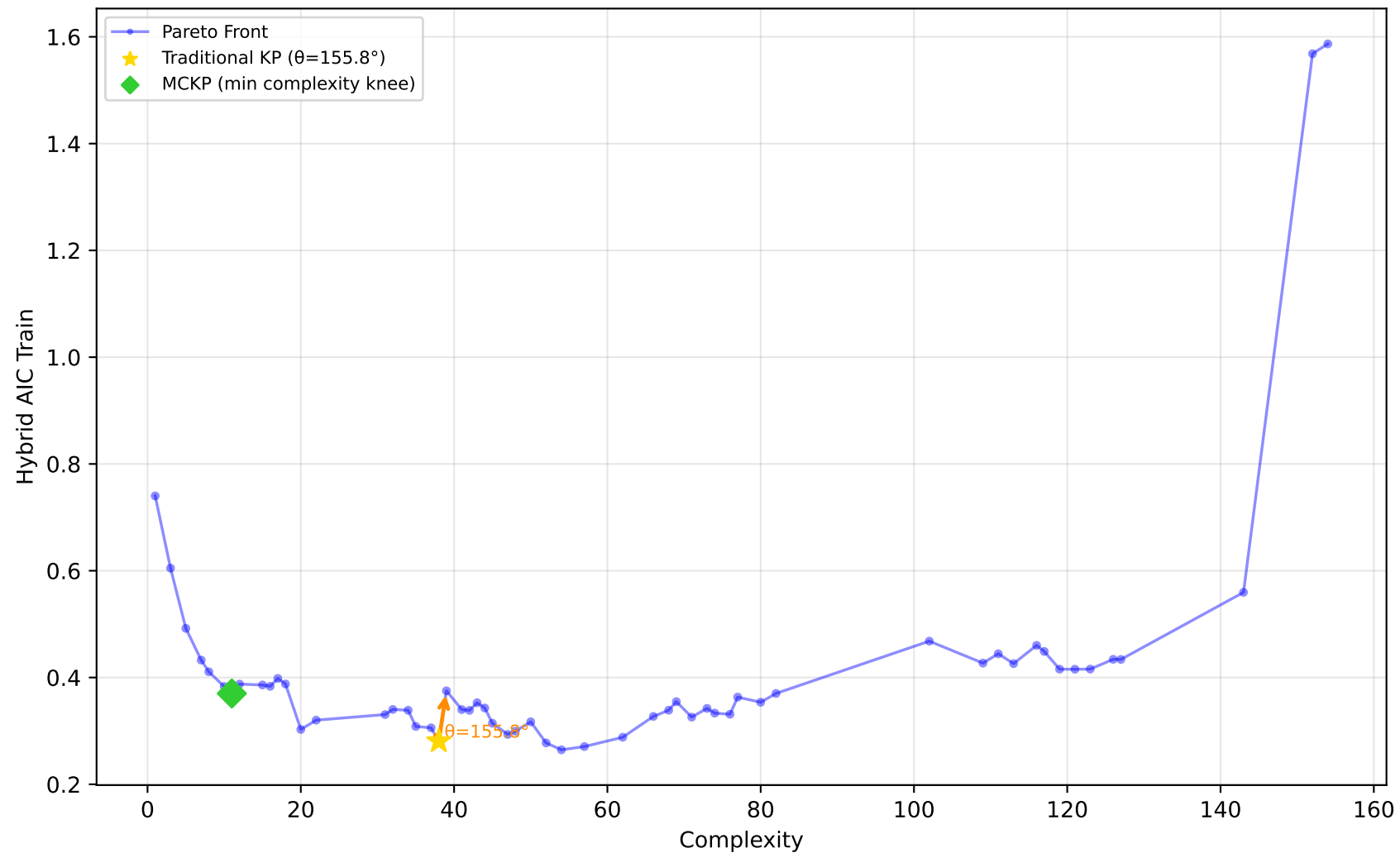
192_vineyard - Run 30 - SVP - Hybrid AIC Train \lambda_1=0.00, \bar{\lambda}_2=1.00, \lambda_3=1.00 | Difficulty: 0.67 | Method: hmr
