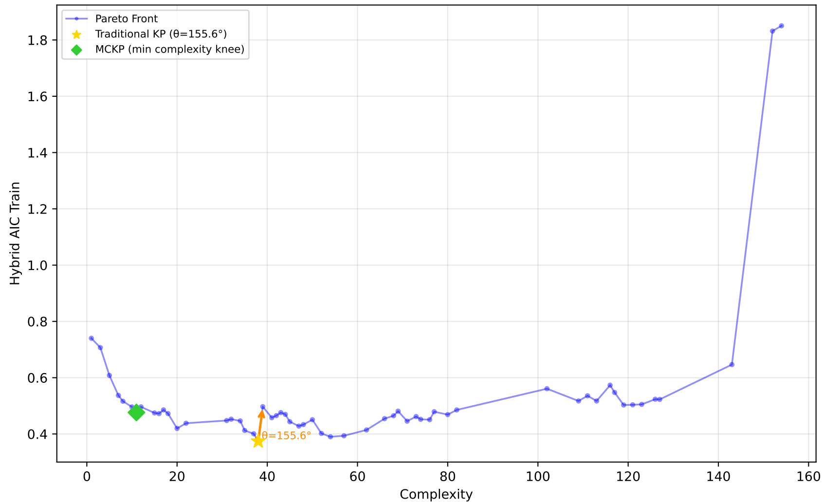
192_vineyard - Run 30 - SVP - Hybrid AIC Train \lambda_1=0.70, \bar{\lambda}_2=0.70, \lambda_3=0.90 | Difficulty: 0.67 | Method: hmr
