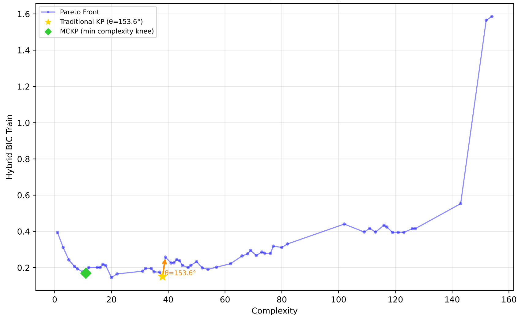
192_vineyard - Run 30 - SVP - Hybrid BIC Train \lambda_1=0.00, \bar{\lambda}_2=1.00, \lambda_3=1.00 | Difficulty: 0.67 | Method: hmr
