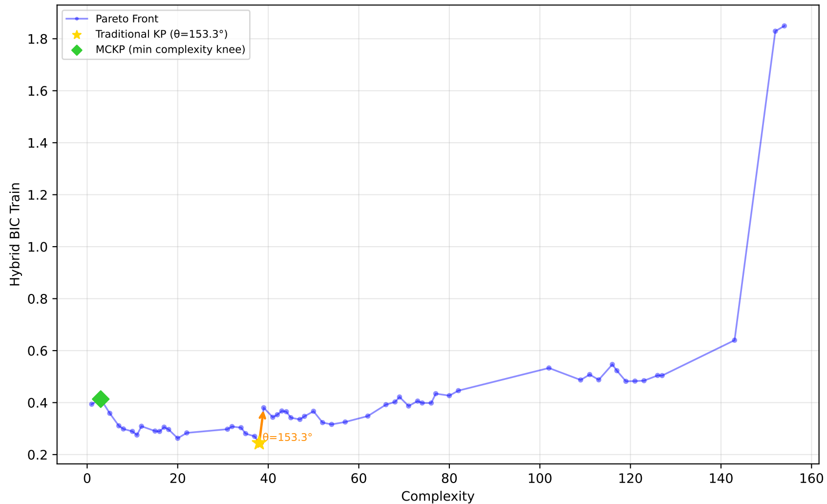
192_vineyard - Run 30 - SVP - Hybrid BIC Train \lambda_1=0.70, \bar{\lambda}_2=0.70, \lambda_3=0.90 | Difficulty: 0.67 | Method: hmr
