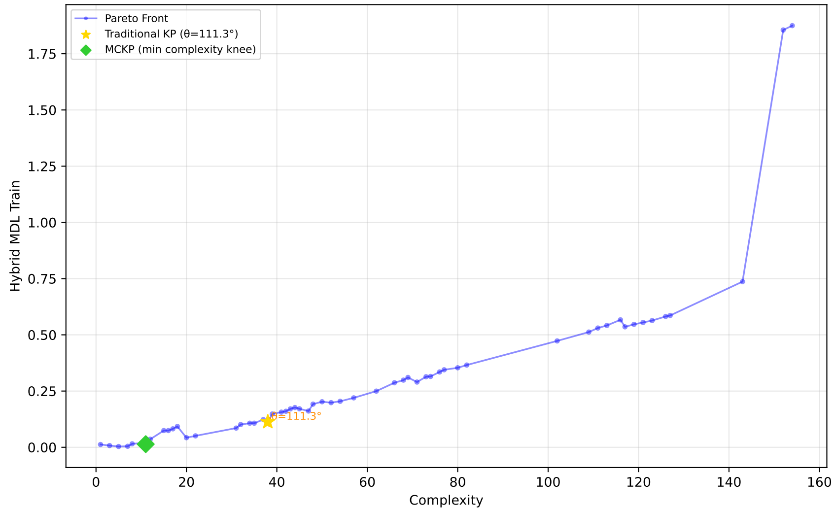
192_vineyard - Run 30 - SVP - Hybrid MDL Train \lambda_1=0.00 , \lambda_2=1.00 , \lambda_3=1.00 | Difficulty: 0.67 | Method: hmr
