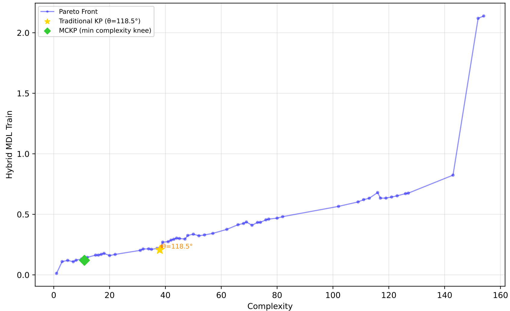
192_vineyard - Run 30 - SVP - Hybrid MDL Train \lambda_1=0.70, \bar{\lambda}_2=0.70, \lambda_3=0.90 | Difficulty: 0.67 | Method: hmr
