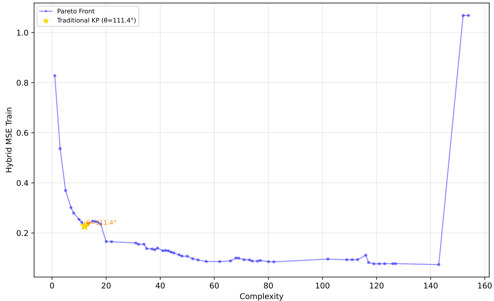
192_vineyard - Run 30 - SVP - Hybrid MSE Train \lambda_1=0.00, \bar{\lambda}_2=1.00, \lambda_3=1.00 | Difficulty: 0.67 | Method: hmr
