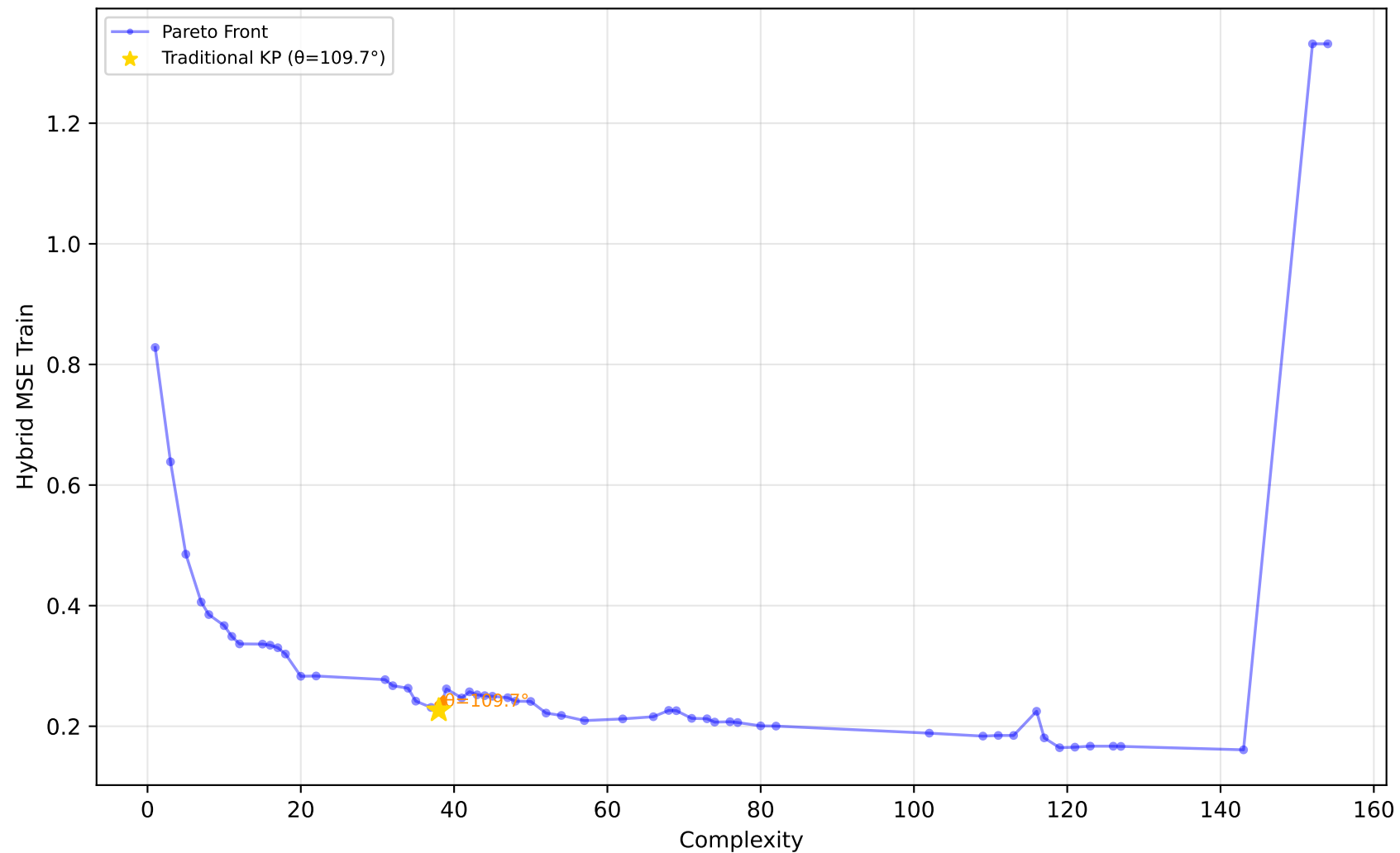
192_vineyard - Run 30 - SVP - Hybrid MSE Train \lambda_1=0.70, \bar{\lambda}_2=0.70, \lambda_3=0.90 | Difficulty: 0.67 | Method: hmr
