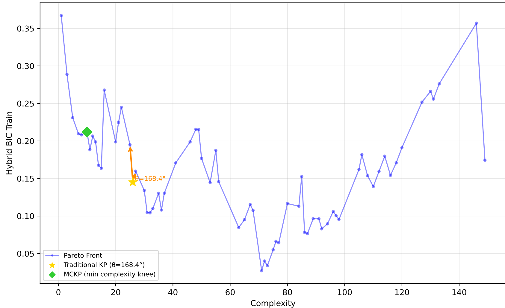
192_vineyard - Run 3 - MVP - Hybrid BIC Train \lambda_1=0.00 , \lambda_2=0.30 , \lambda_3=1.00 | Difficulty: 1.00 | Method: hmr
