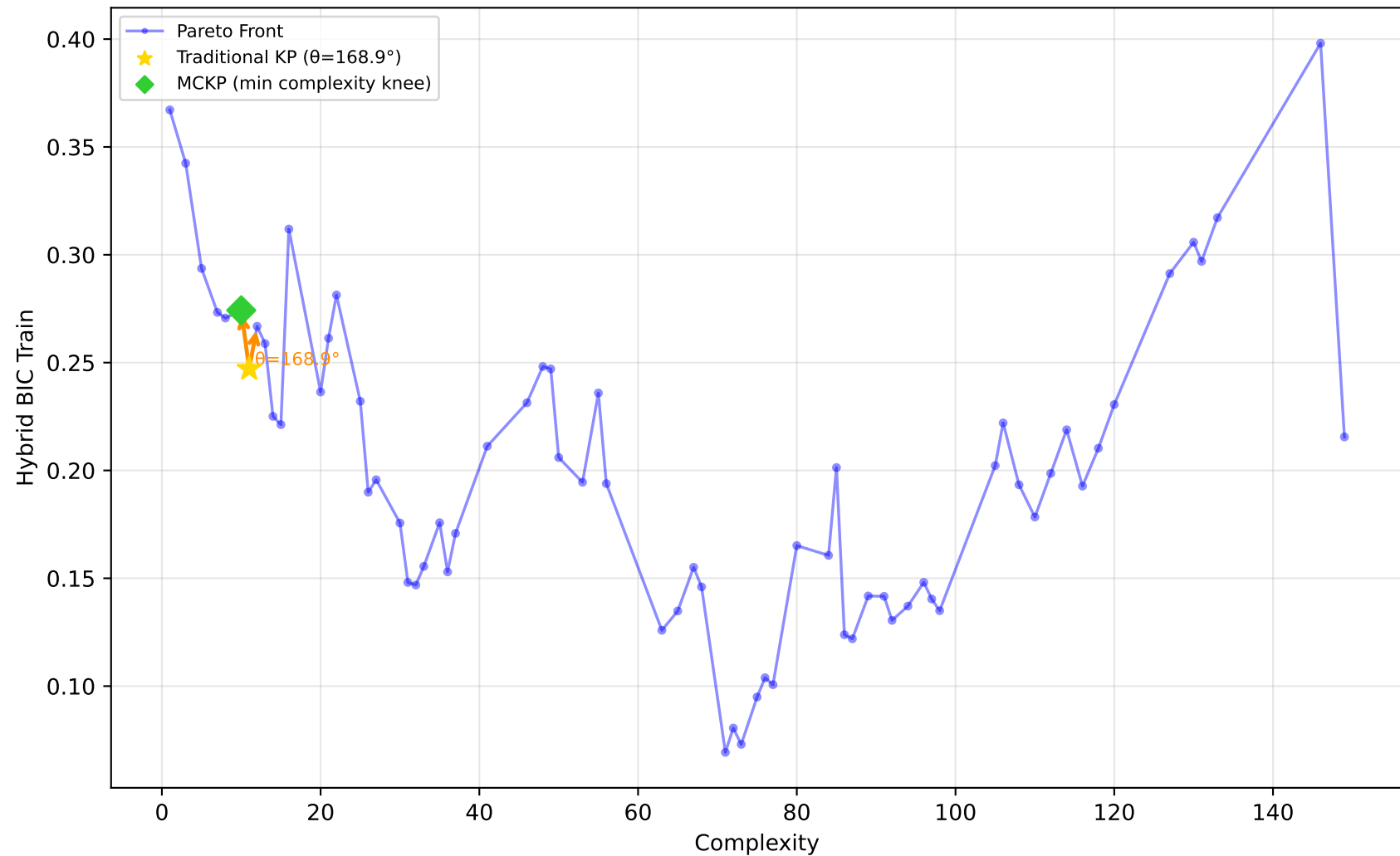
192_vineyard - Run 3 - MVP - Hybrid BIC Train \lambda_1=0.40, \lambda_2=0.00, \lambda_3=1.00 | Difficulty: 1.00 | Method: hmr
