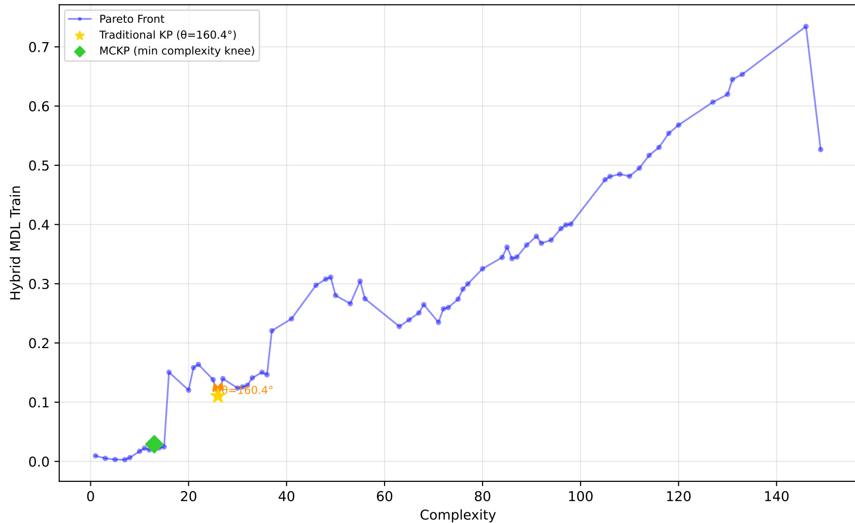
192_vineyard - Run 3 - MVP - Hybrid MDL Train \lambda_1=0.00, \bar{\lambda}_2=0.30, \lambda_3=1.00 | Difficulty: 1.00 | Method: hmr
