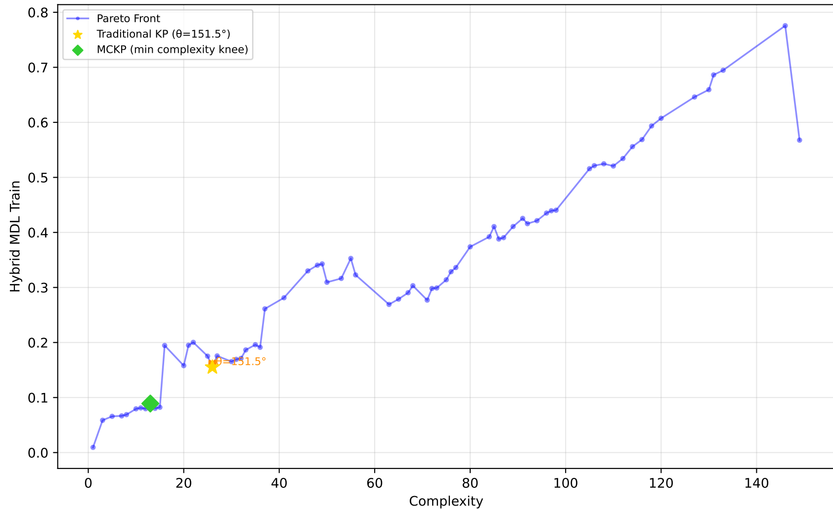
192_vineyard - Run 3 - MVP - Hybrid MDL Train \lambda_1=0.40, \bar{\lambda}_2=0.00, \lambda_3=1.00 | Difficulty: 1.00 | Method: hmr
