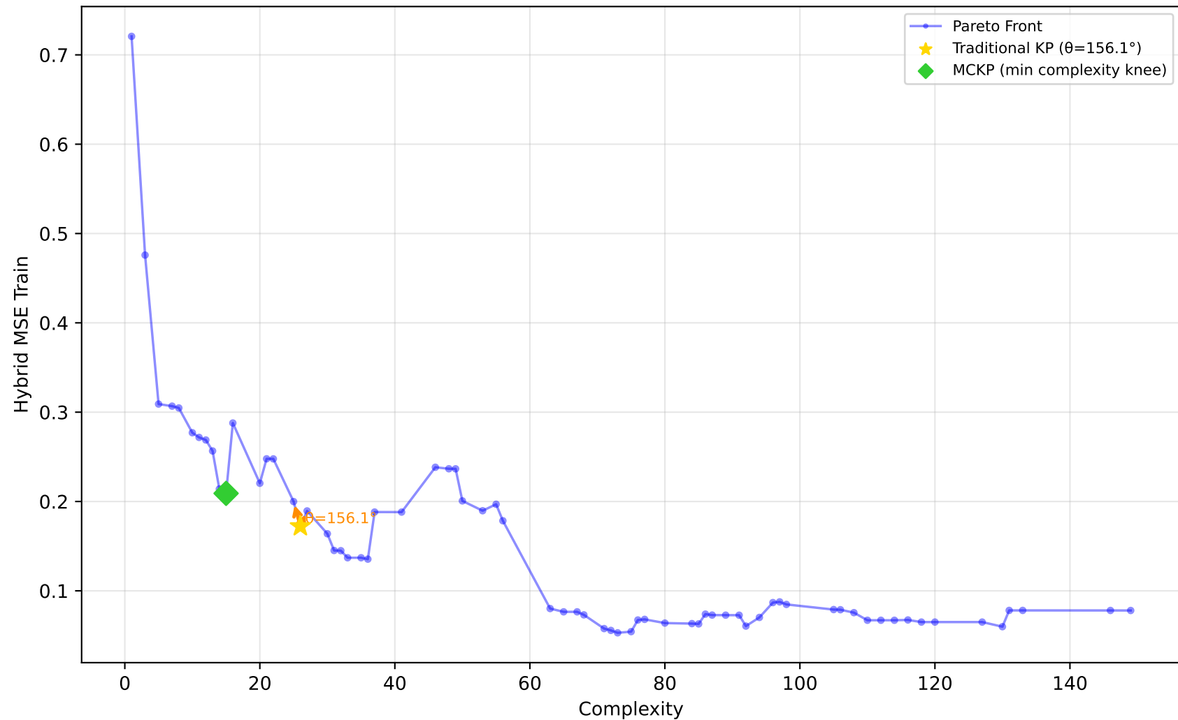
192_vineyard - Run 3 - MVP - Hybrid MSE Train \lambda_1=0.00, \bar{\lambda}_2=0.30, \lambda_3=1.00 | Difficulty: 1.00 | Method: hmr
