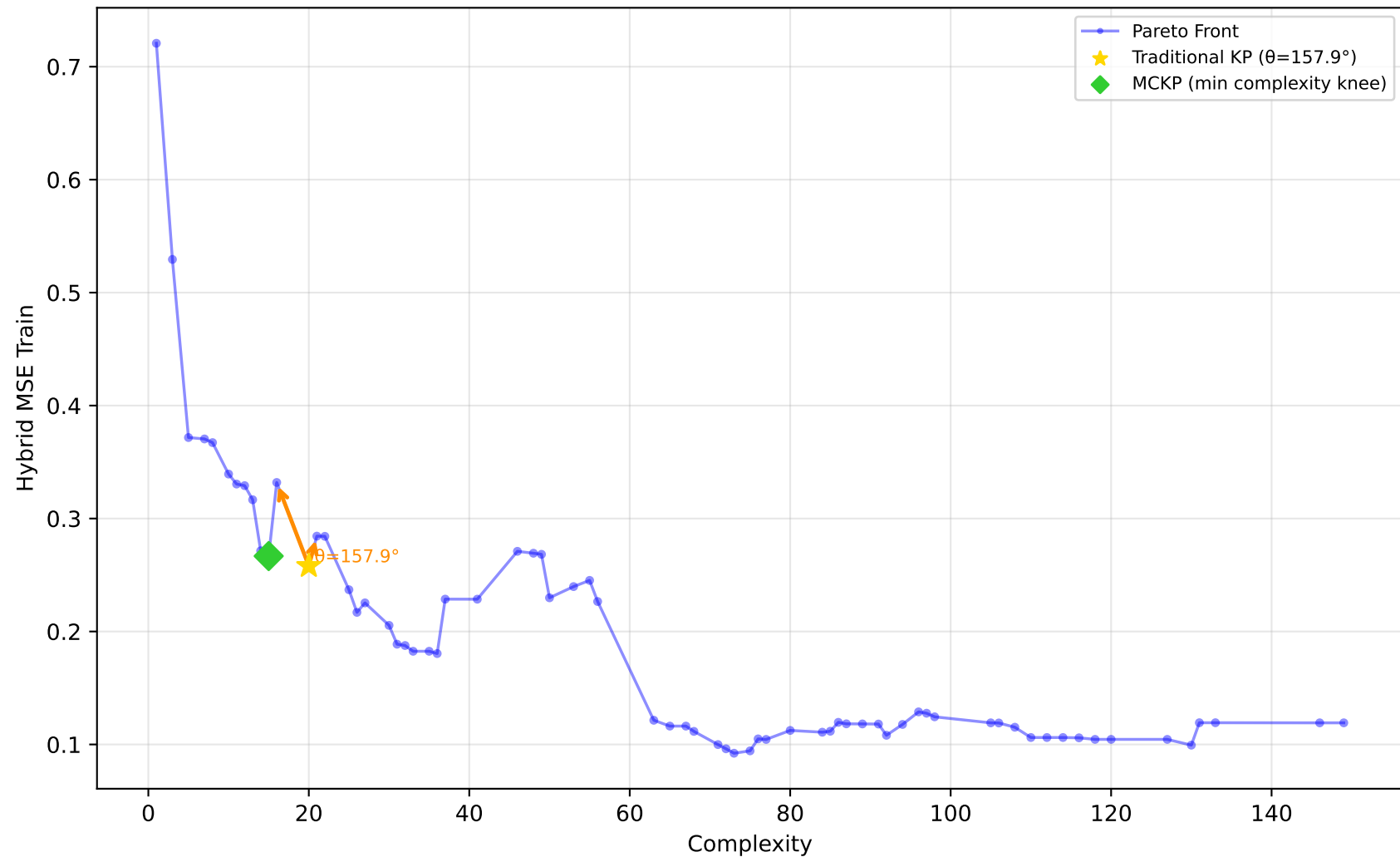
192_vineyard - Run 3 - MVP - Hybrid MSE Train \lambda_1=0.40, \bar{\lambda}_2=0.00, \lambda_3=1.00 | Difficulty: 1.00 | Method: hmr
