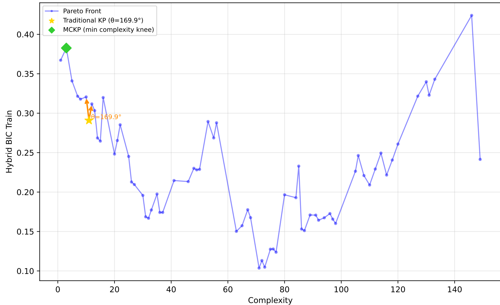
192_vineyard - Run 3 - SVP - Hybrid BIC Train \lambda_1=0.70, \lambda_2=0.70, \lambda_3=0.90 | Difficulty: 1.00 | Method: hmr
