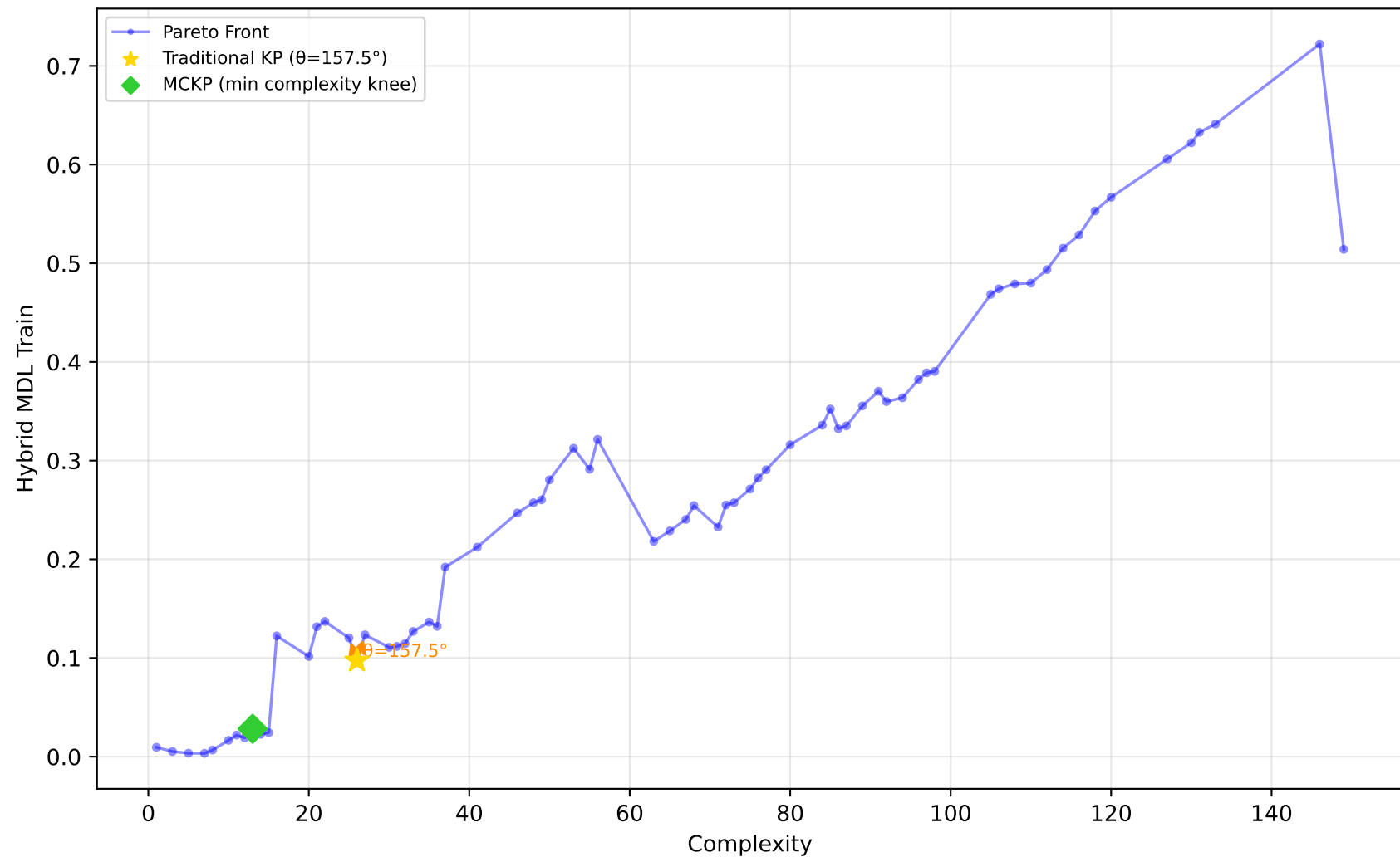
192_vineyard - Run 3 - SVP - Hybrid MDL Train \lambda_1=0.00, \bar{\lambda}_2=1.00, \lambda_3=1.00 | Difficulty: 1.00 | Method: hmr
