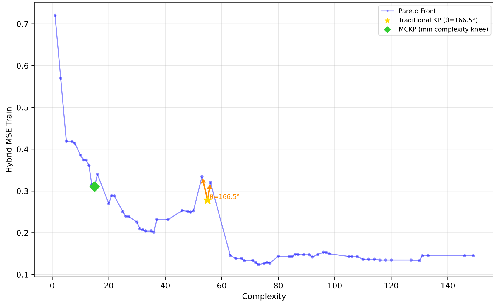
192_vineyard - Run 3 - SVP - Hybrid MSE Train \lambda_1=0.70, \bar{\lambda}_2=0.70, \lambda_3=0.90 | Difficulty: 1.00 | Method: hmr
