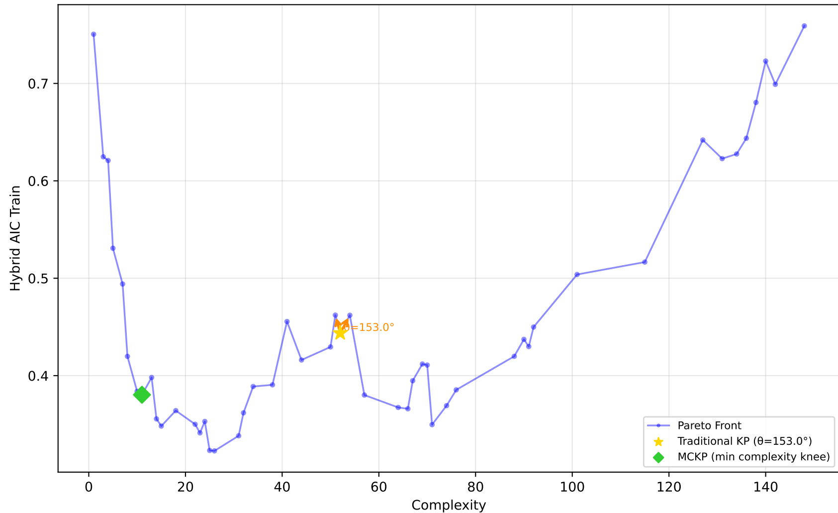
192_vineyard - Run 4 - MVP - Hybrid AIC Train \lambda_1=0.00, \lambda_2=0.30, \lambda_3=1.00 | Difficulty: 1.00 | Method: hmr
