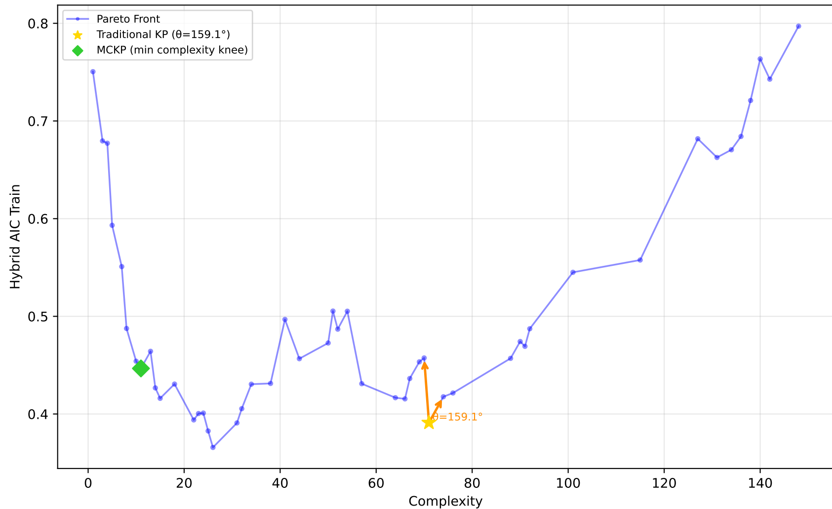
192_vineyard - Run 4 - MVP - Hybrid AIC Train \lambda_1=0.40, \lambda_2=0.00, \lambda_3=1.00 | Difficulty: 1.00 | Method: hmr
