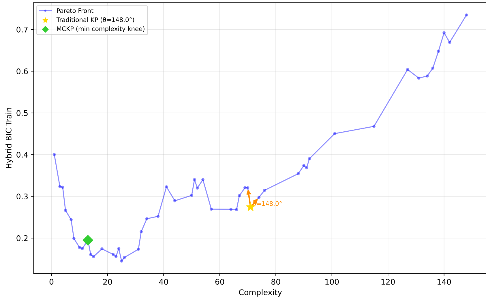
192_vineyard - Run 4 - MVP - Hybrid BIC Train \lambda_1=0.00, \lambda_2=0.30, \lambda_3=1.00 | Difficulty: 1.00 | Method: hmr
