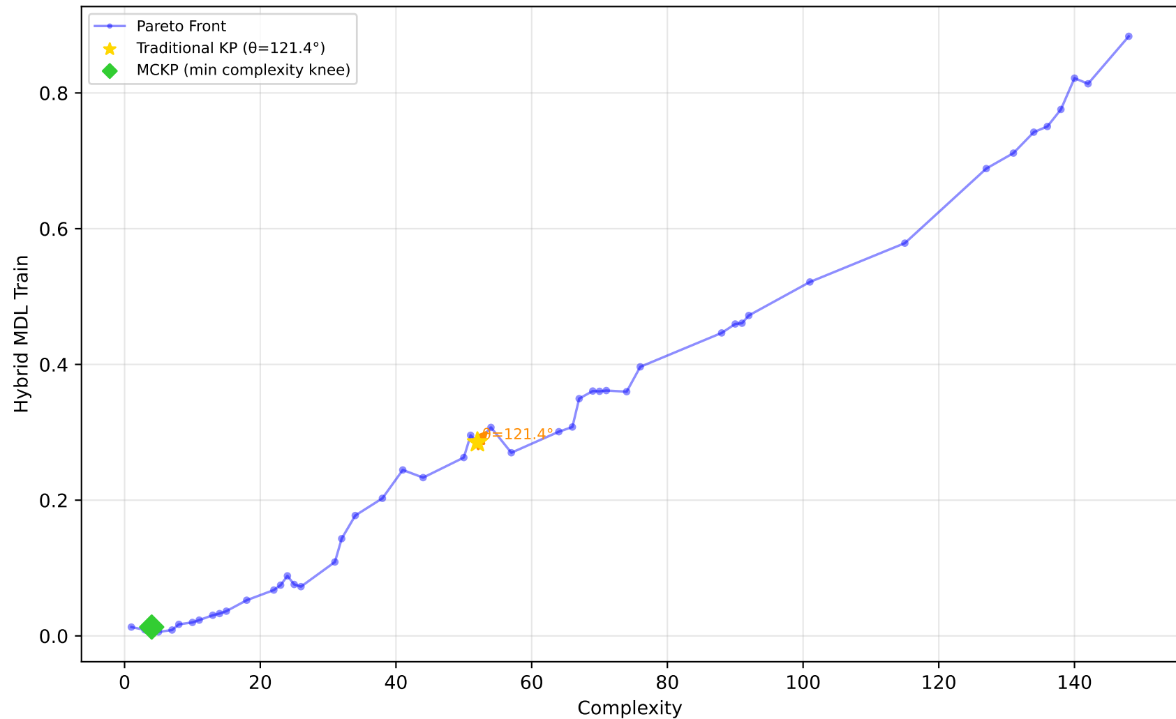
192_vineyard - Run 4 - MVP - Hybrid MDL Train \lambda_1=0.00, \bar{\lambda}_2=0.30, \lambda_3=1.00 | Difficulty: 1.00 | Method: hmr
