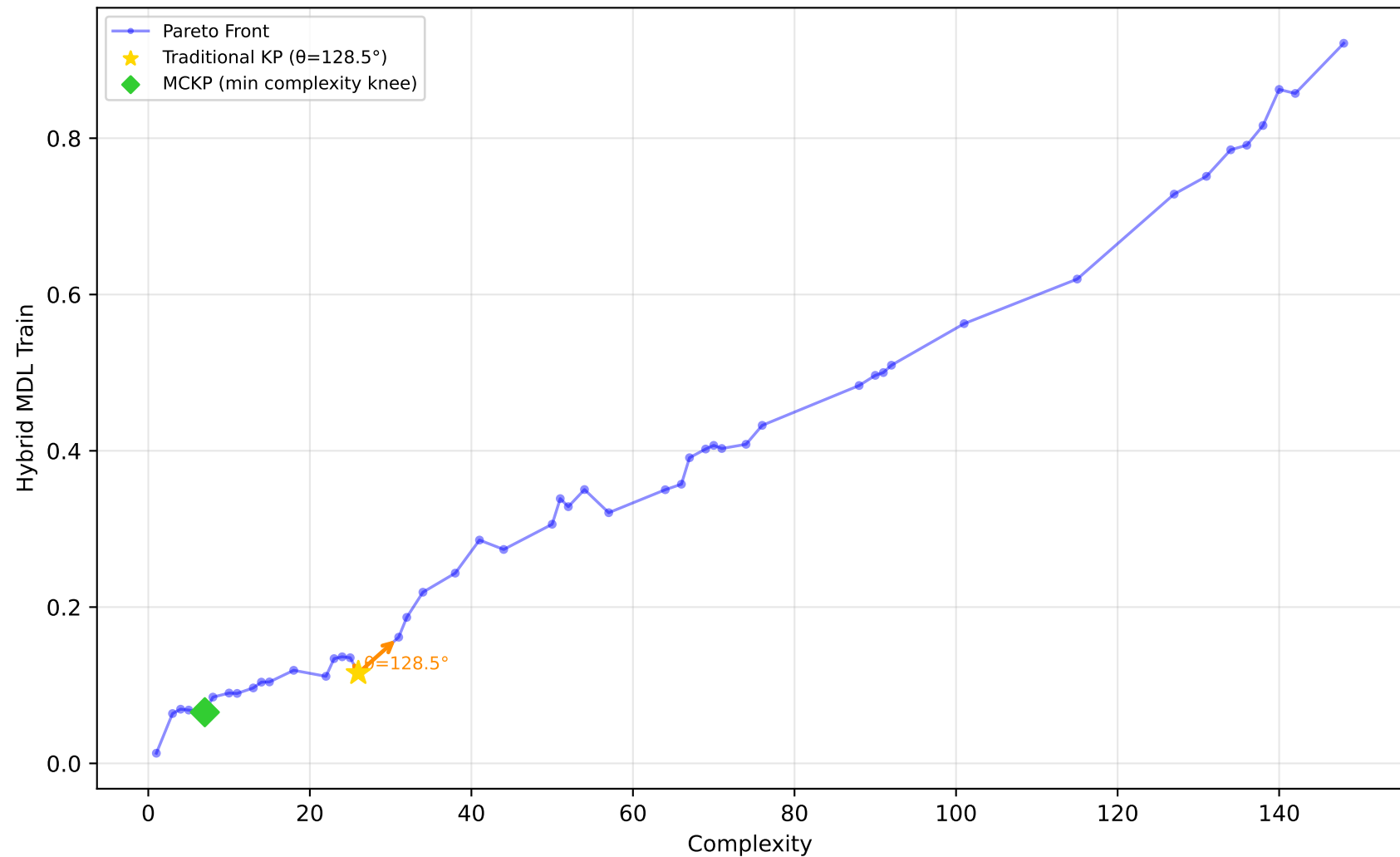
192_vineyard - Run 4 - MVP - Hybrid MDL Train \lambda_1=0.40, \bar{\lambda}_2=0.00, \lambda_3=1.00 | Difficulty: 1.00 | Method: hmr
