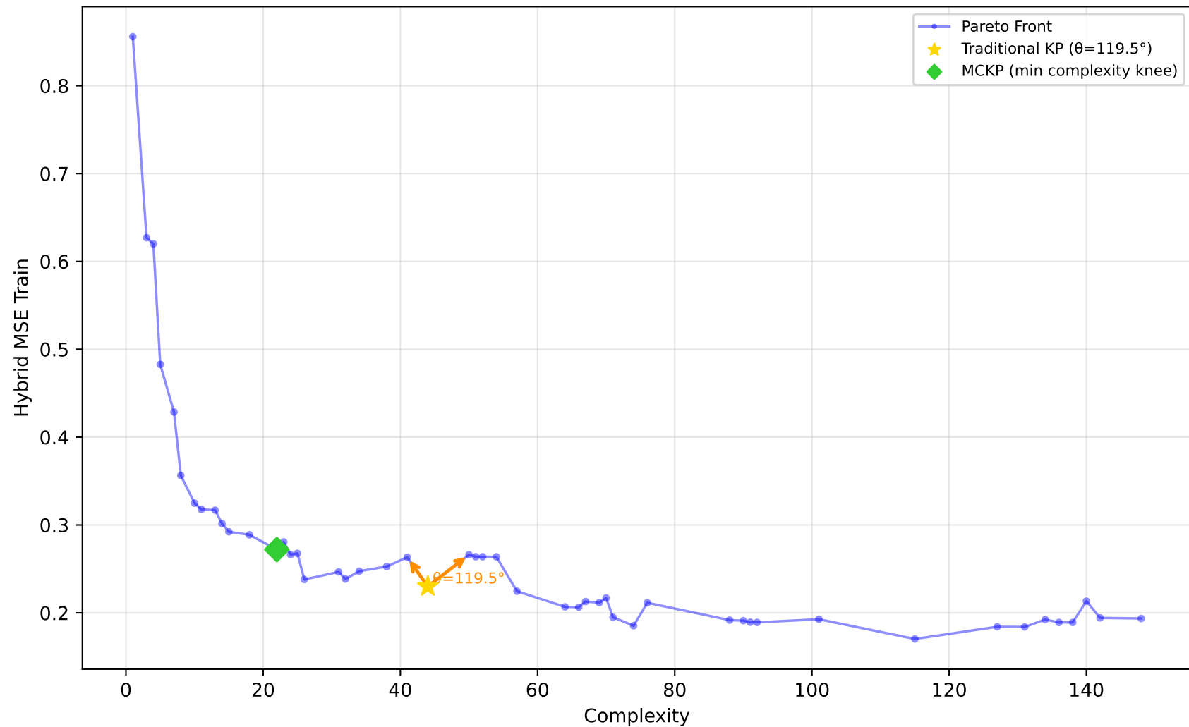
192_vineyard - Run 4 - MVP - Hybrid MSE Train \lambda_1=0.40, \bar{\lambda}_2=0.00, \lambda_3=1.00 | Difficulty: 1.00 | Method: hmr
