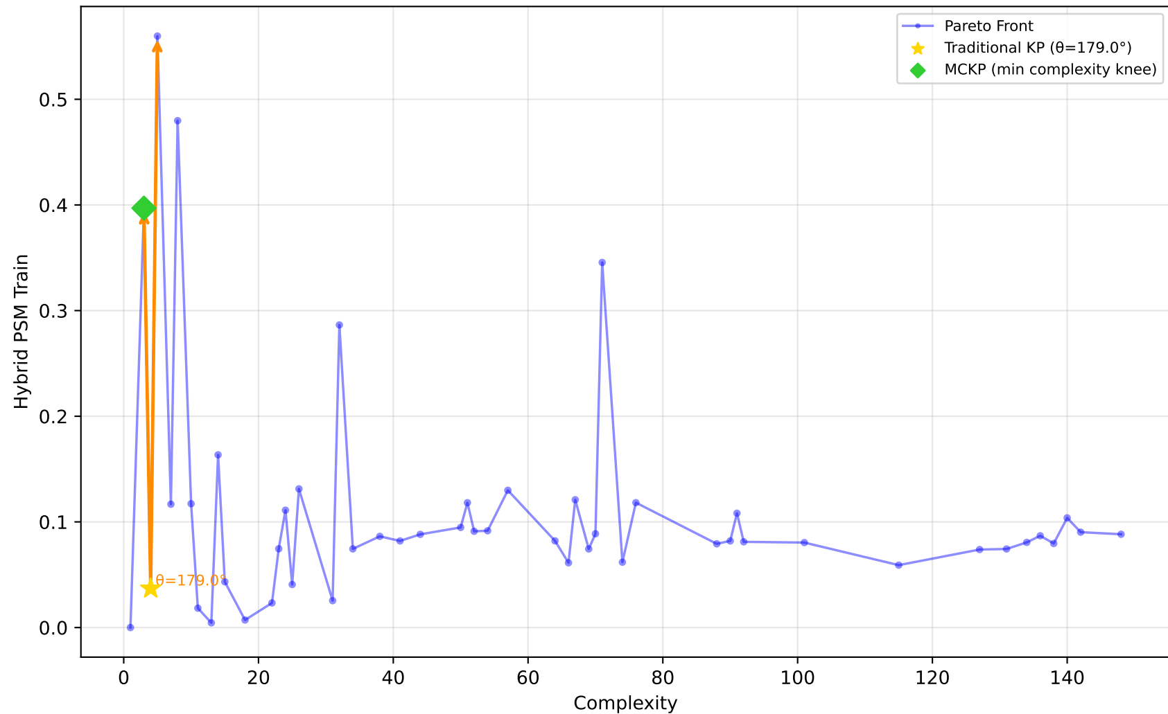
192_vineyard - Run 4 - MVP - Hybrid PSM Train \lambda_1=0.00, \bar{\lambda}_2=0.30, \lambda_3=1.00 | Difficulty: 1.00 | Method: hmr
