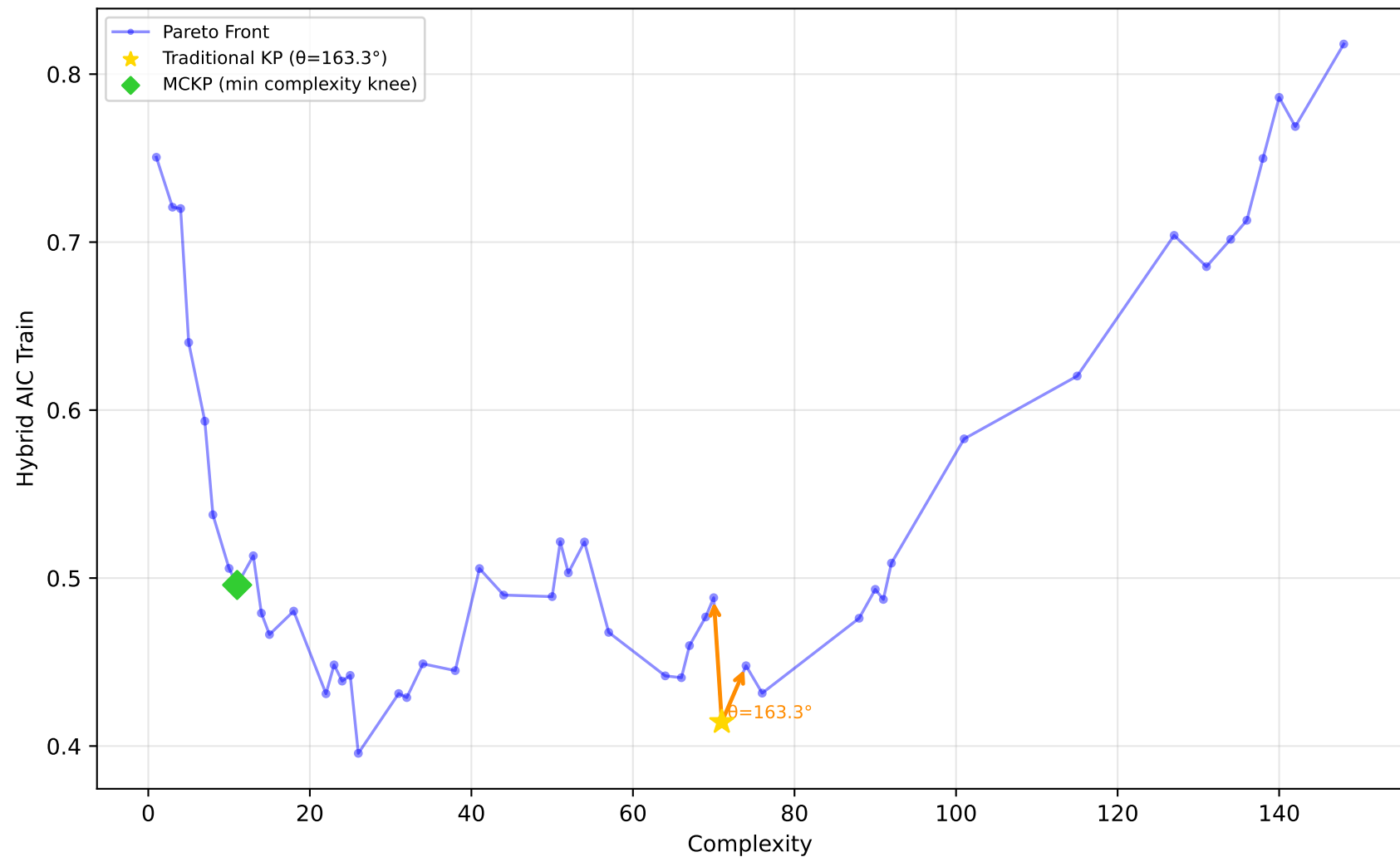
192_vineyard - Run 4 - SVP - Hybrid AIC Train \lambda_1=0.70, \lambda_2=0.70, \lambda_3=0.90 | Difficulty: 1.00 | Method: hmr
