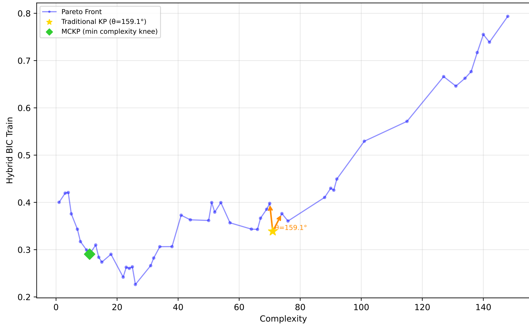
192_vineyard - Run 4 - SVP - Hybrid BIC Train \lambda_1=0.70, \lambda_2=0.70, \lambda_3=0.90 | Difficulty: 1.00 | Method: hmr
