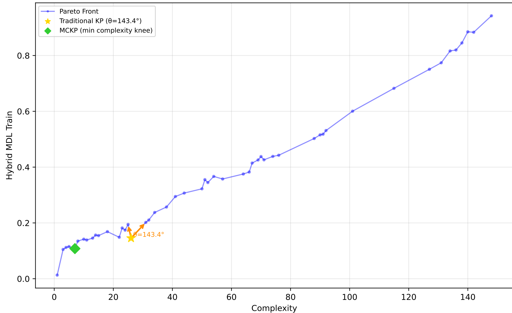
192_vineyard - Run 4 - SVP - Hybrid MDL Train \lambda_1=0.70, \bar{\lambda}_2=0.70, \lambda_3=0.90 | Difficulty: 1.00 | Method: hmr
