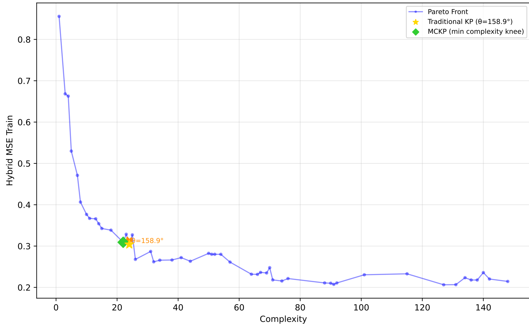
192_vineyard - Run 4 - SVP - Hybrid MSE Train \lambda_1=0.70, \bar{\lambda}_2=0.70, \lambda_3=0.90 | Difficulty: 1.00 | Method: hmr
