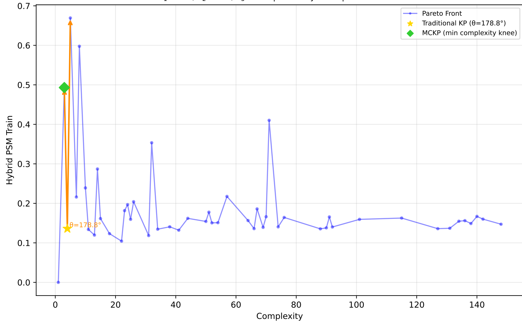
192_vineyard - Run 4 - SVP - Hybrid PSM Train \lambda_1=0.70, \lambda_2=0.70, \lambda_3=0.90 | Difficulty: 1.00 | Method: hmr
