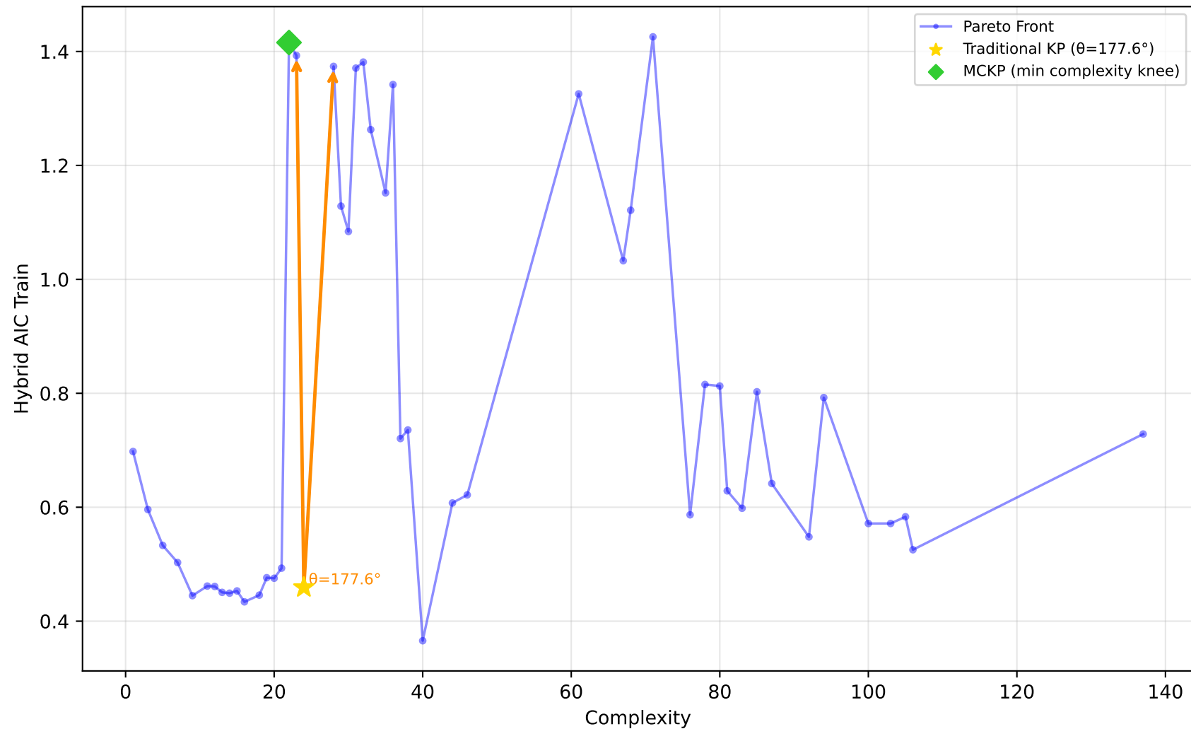
192_vineyard - Run 5 - MVP - Hybrid AIC Train \lambda_1=0.00, \lambda_2=0.30, \lambda_3=1.00 | Difficulty: 1.00 | Method: hmr
