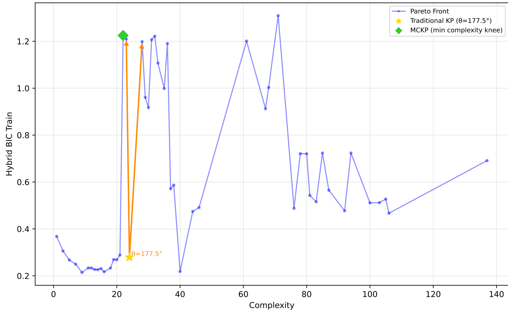
192_vineyard - Run 5 - MVP - Hybrid BIC Train \lambda_1=0.00, \lambda_2=0.30, \lambda_3=1.00 | Difficulty: 1.00 | Method: hmr
