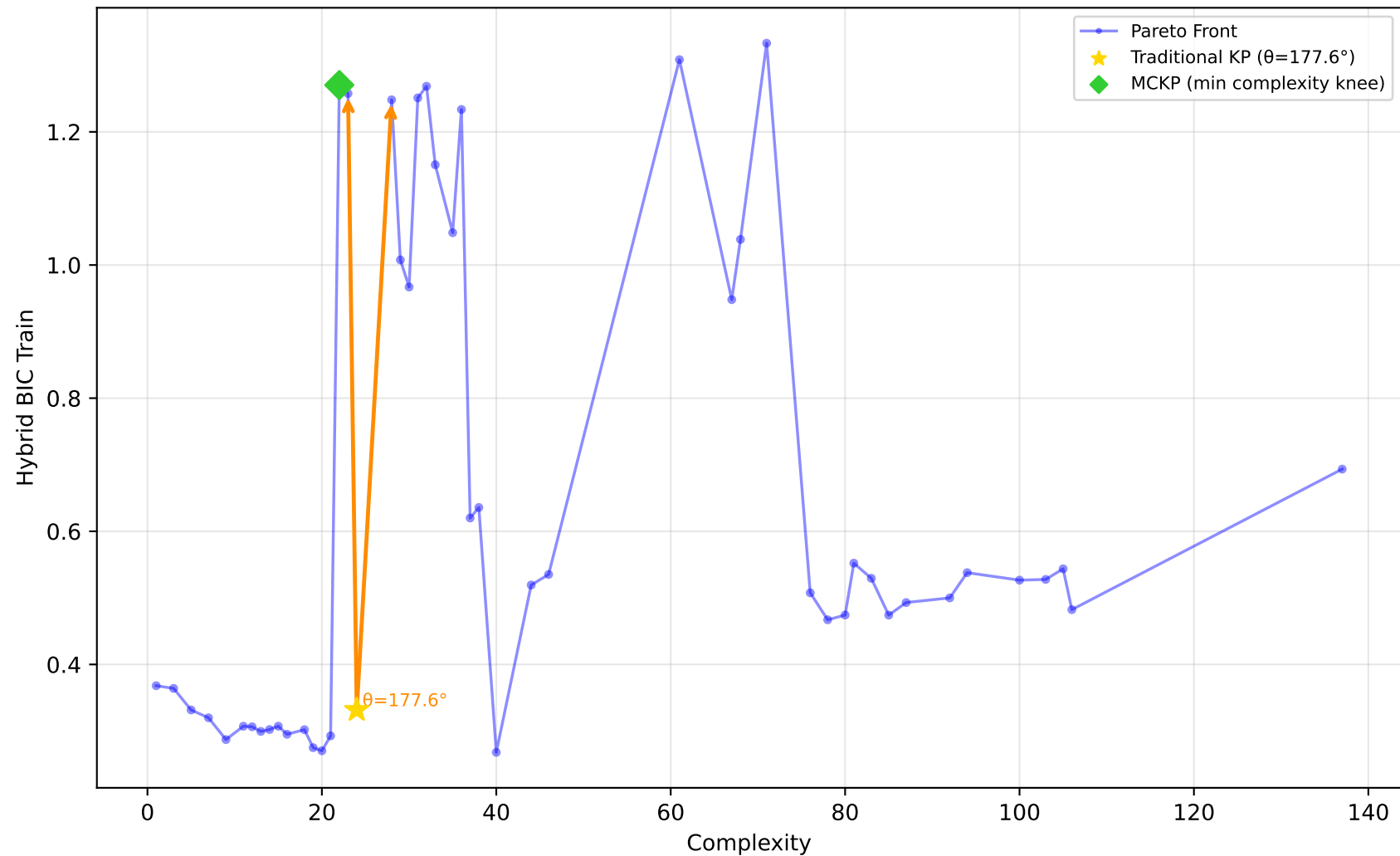
192_vineyard - Run 5 - MVP - Hybrid BIC Train \lambda_1=0.40, \lambda_2=0.00, \lambda_3=1.00 | Difficulty: 1.00 | Method: hmr
