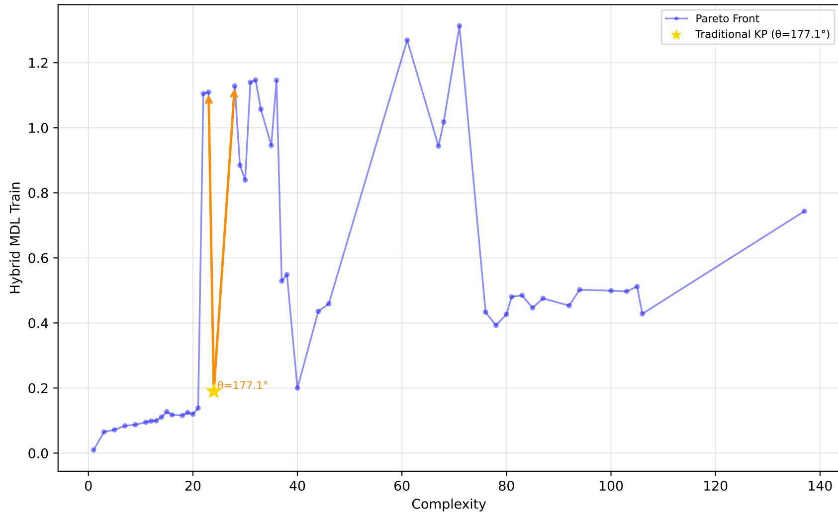
192_vineyard - Run 5 - MVP - Hybrid MDL Train \lambda_1=0.40, \bar{\lambda}_2=0.00, \lambda_3=1.00 | Difficulty: 1.00 | Method: hmr
