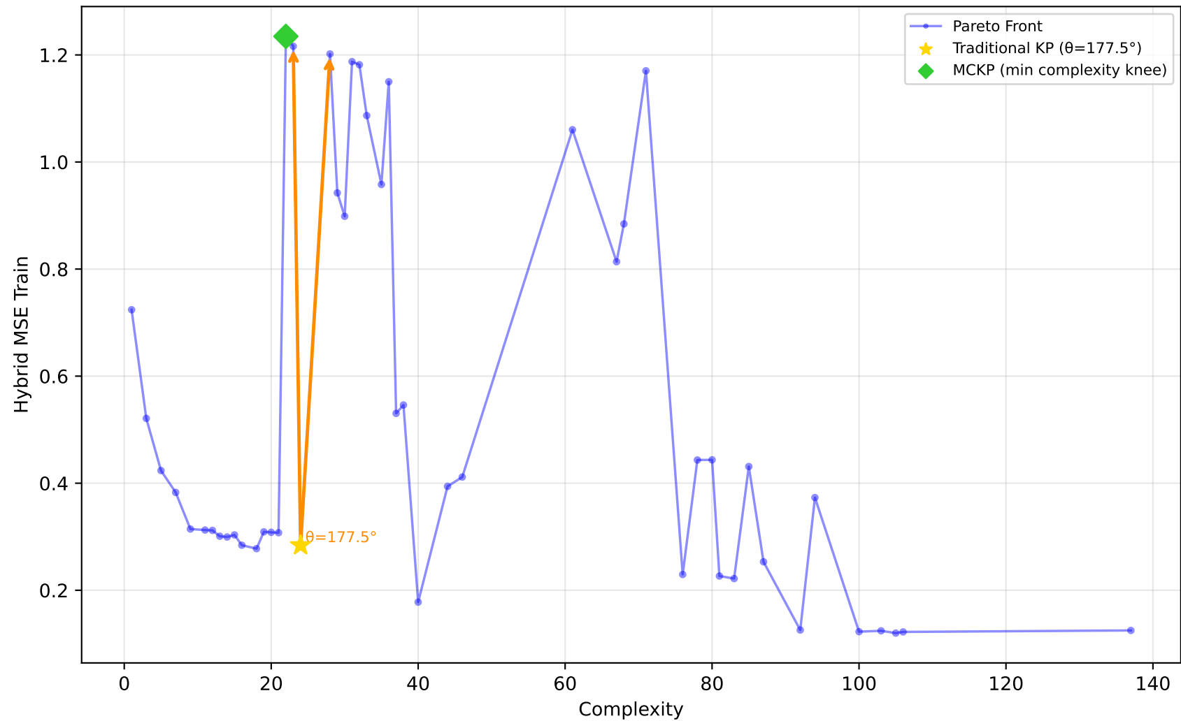
192_vineyard - Run 5 - MVP - Hybrid MSE Train \lambda_1=0.00, \bar{\lambda}_2=0.30, \lambda_3=1.00 | Difficulty: 1.00 | Method: hmr
