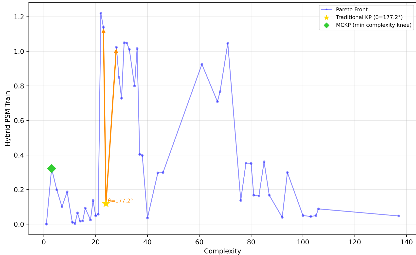
192_vineyard - Run 5 - MVP - Hybrid PSM Train \lambda_1=0.00, \bar{\lambda}_2=0.30, \lambda_3=1.00 | Difficulty: 1.00 | Method: hmr
