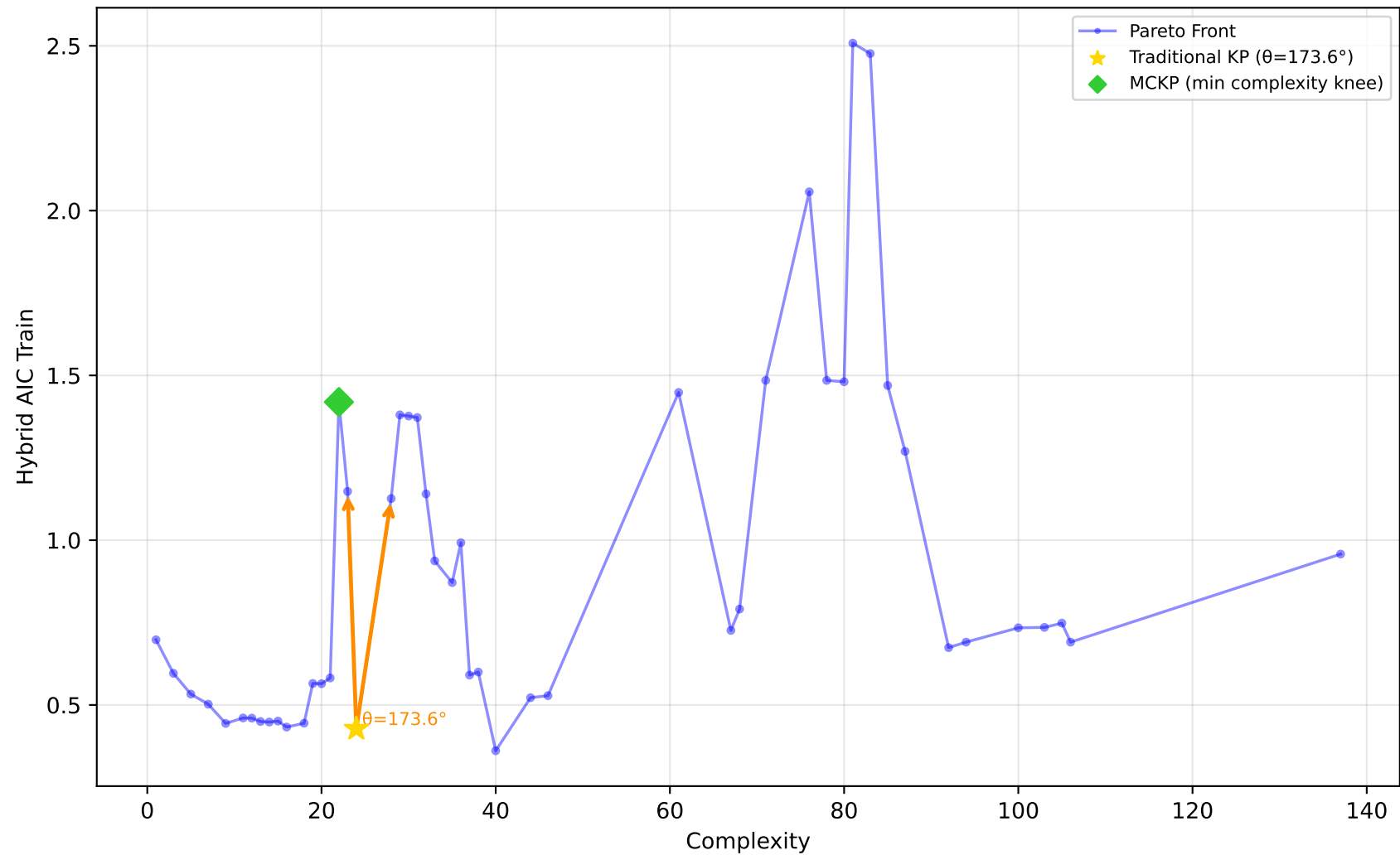
192_vineyard - Run 5 - SVP - Hybrid AIC Train \lambda_1=0.00, \lambda_2=1.00, \lambda_3=1.00 | Difficulty: 1.00 | Method: hmr
