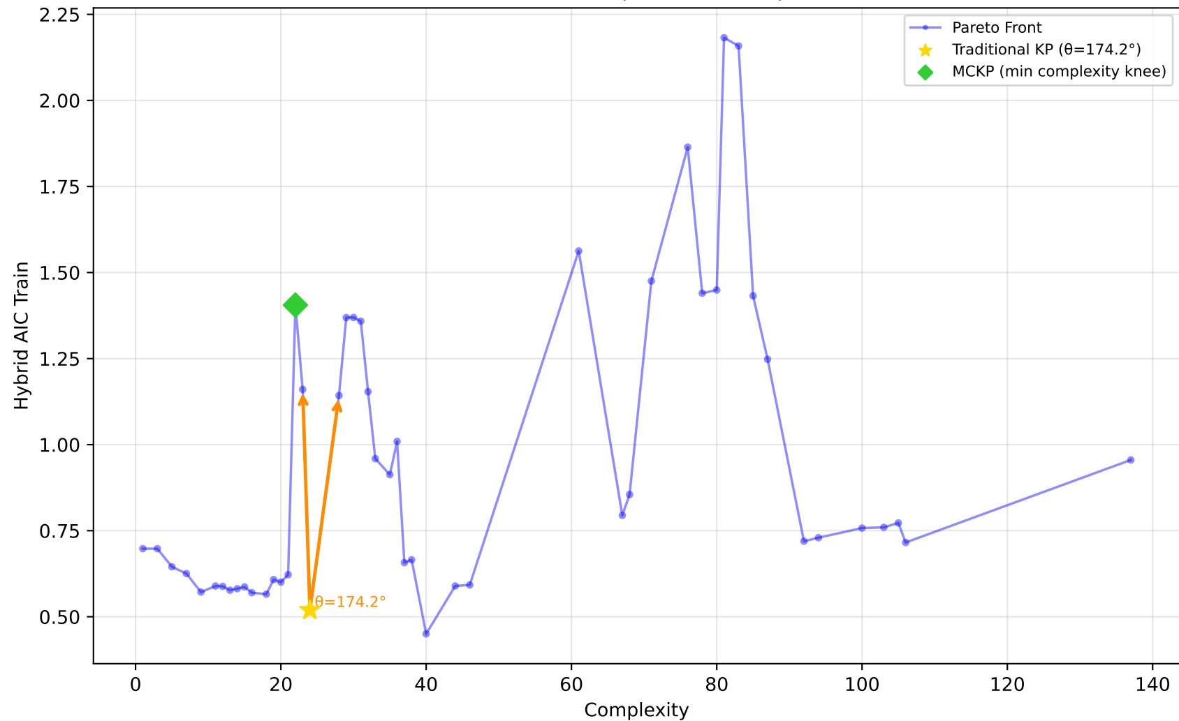
192_vineyard - Run 5 - SVP - Hybrid AIC Train \lambda_1=0.70, \lambda_2=0.70, \lambda_3=0.90 | Difficulty: 1.00 | Method: hmr
