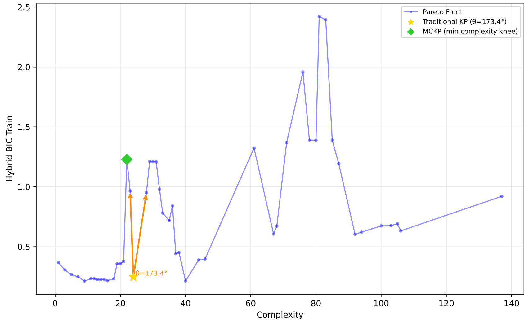
192_vineyard - Run 5 - SVP - Hybrid BIC Train \lambda_1=0.00, \lambda_2=1.00, \lambda_3=1.00 | Difficulty: 1.00 | Method: hmr
