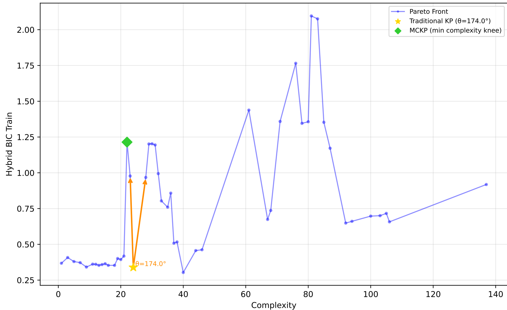
192_vineyard - Run 5 - SVP - Hybrid BIC Train \lambda_1=0.70 , \lambda_2=0.70 , \lambda_3=0.90 | Difficulty: 1.00 | Method: hmr
