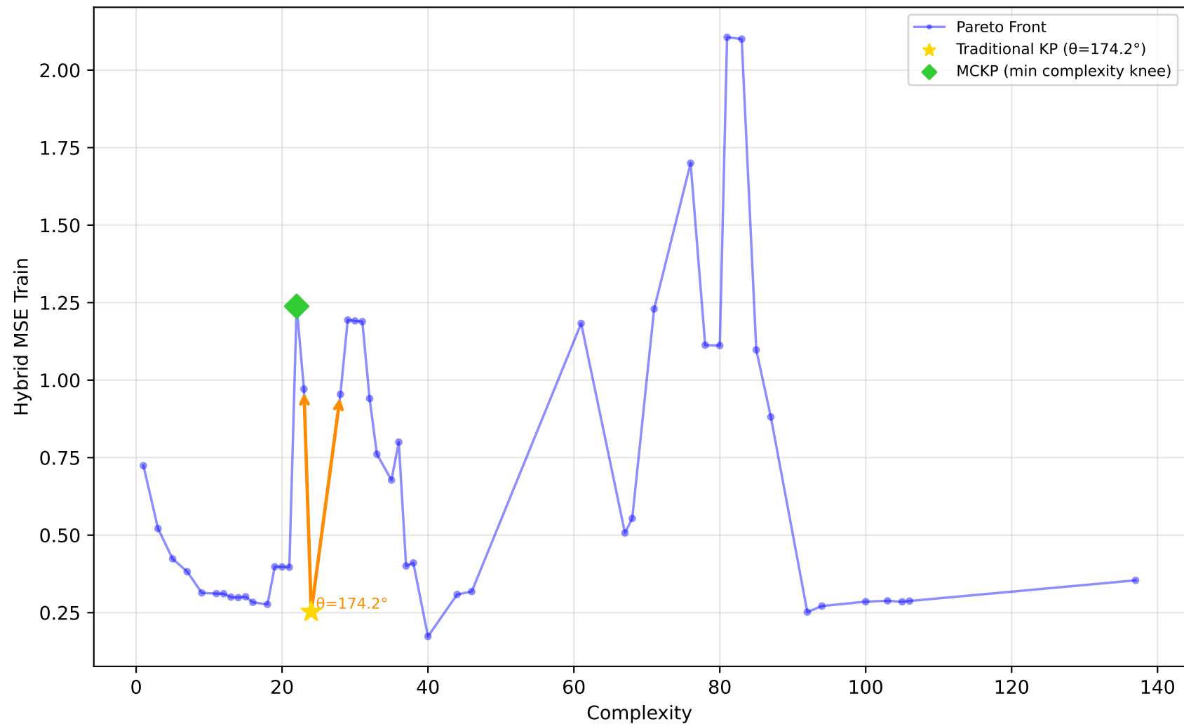
192_vineyard - Run 5 - SVP - Hybrid MSE Train \lambda_1=0.00 , \lambda_2=1.00 , \lambda_3=1.00 | Difficulty: 1.00 | Method: hmr
