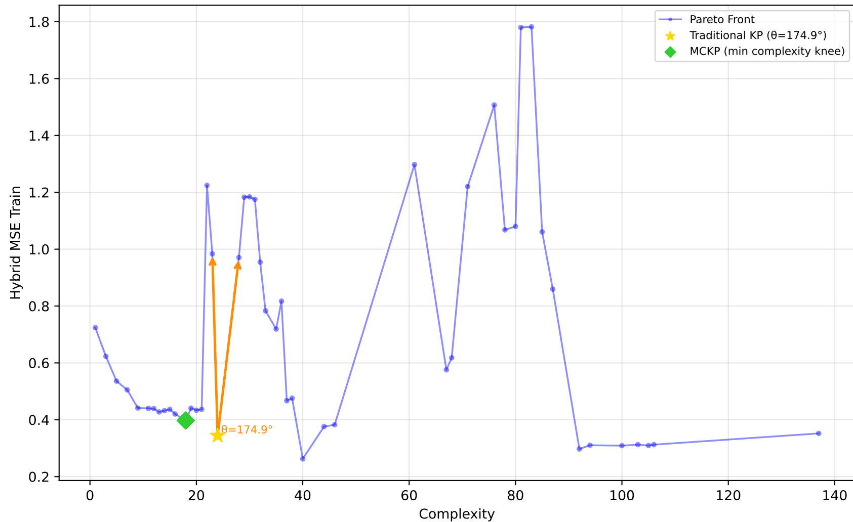
192_vineyard - Run 5 - SVP - Hybrid MSE Train \lambda_1=0.70, \lambda_2=0.70, \lambda_3=0.90 | Difficulty: 1.00 | Method: hmr
