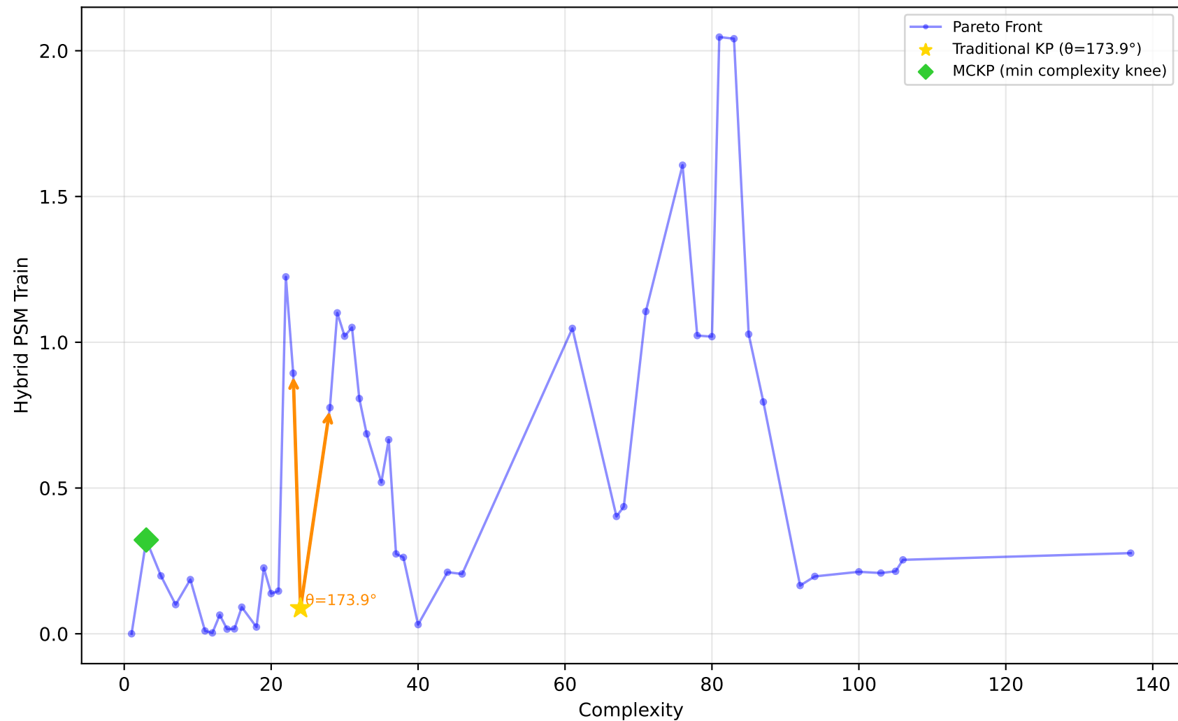
192_vineyard - Run 5 - SVP - Hybrid PSM Train \lambda_1=0.00, \bar{\lambda}_2=1.00, \lambda_3=1.00 | Difficulty: 1.00 | Method: hmr
