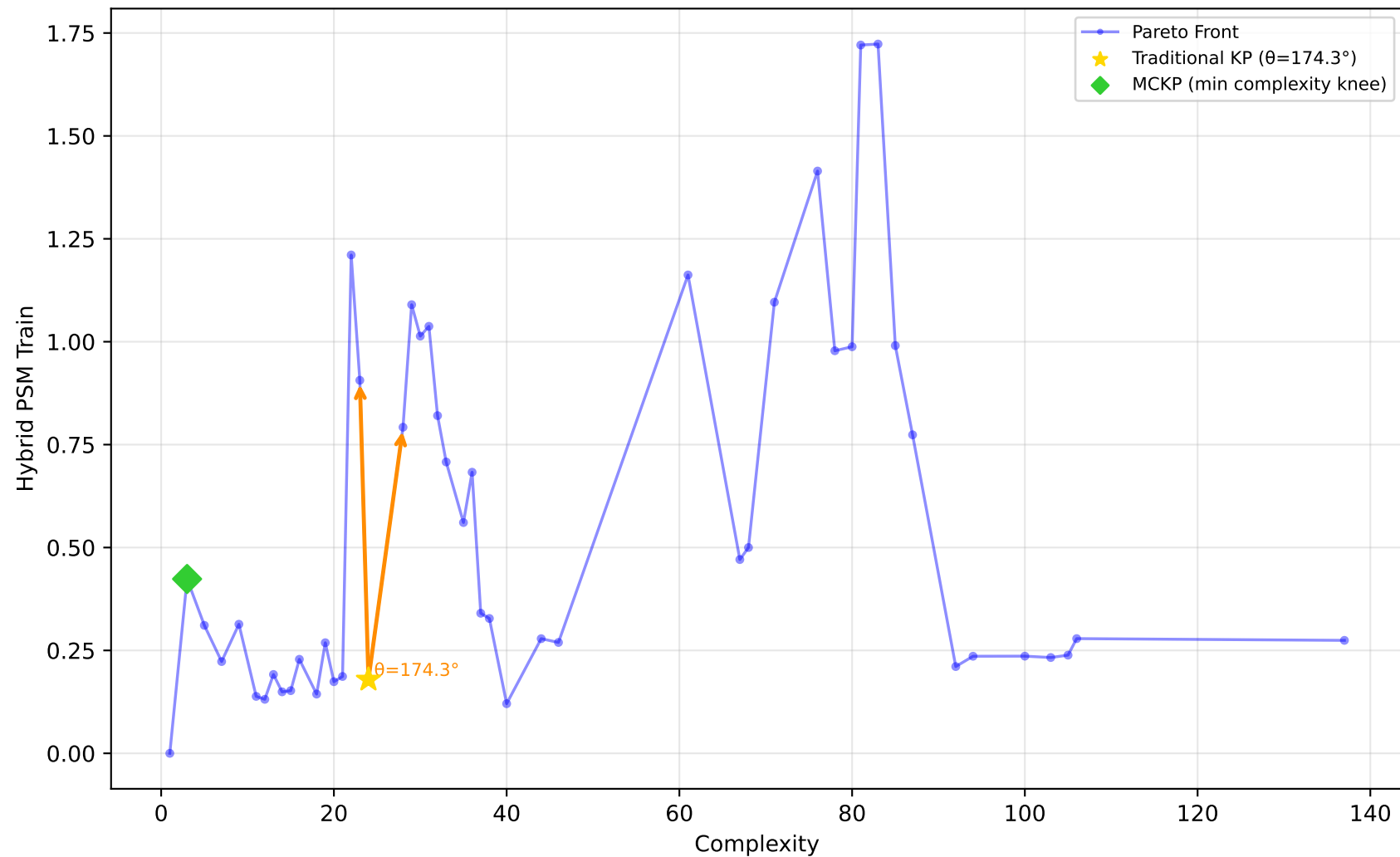
192_vineyard - Run 5 - SVP - Hybrid PSM Train \lambda_1=0.70 , \lambda_2=0.70 , \lambda_3=0.90 | Difficulty: 1.00 | Method: hmr
