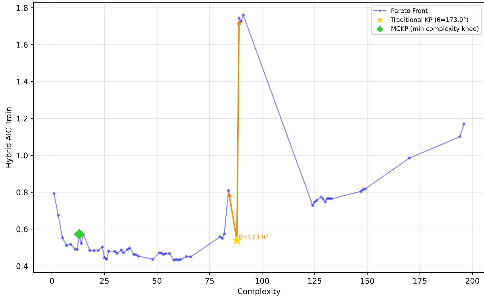
192_vineyard - Run 6 - MVP - Hybrid AIC Train \lambda_1=0.00, \lambda_2=0.30, \lambda_3=1.00 | Difficulty: 1.00 | Method: hmr
